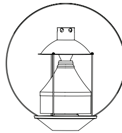
RG-25. /OPAS.RL Reflector Optics (acrylic sphere)
