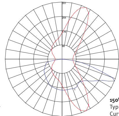
70W HPS Typical Polar Curve
