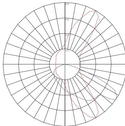
150W HPS Typical Polar Curve
